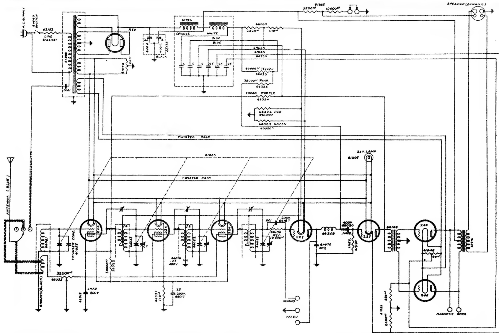
Stewart-Warner 950 Series A. C. Radio Receivers
