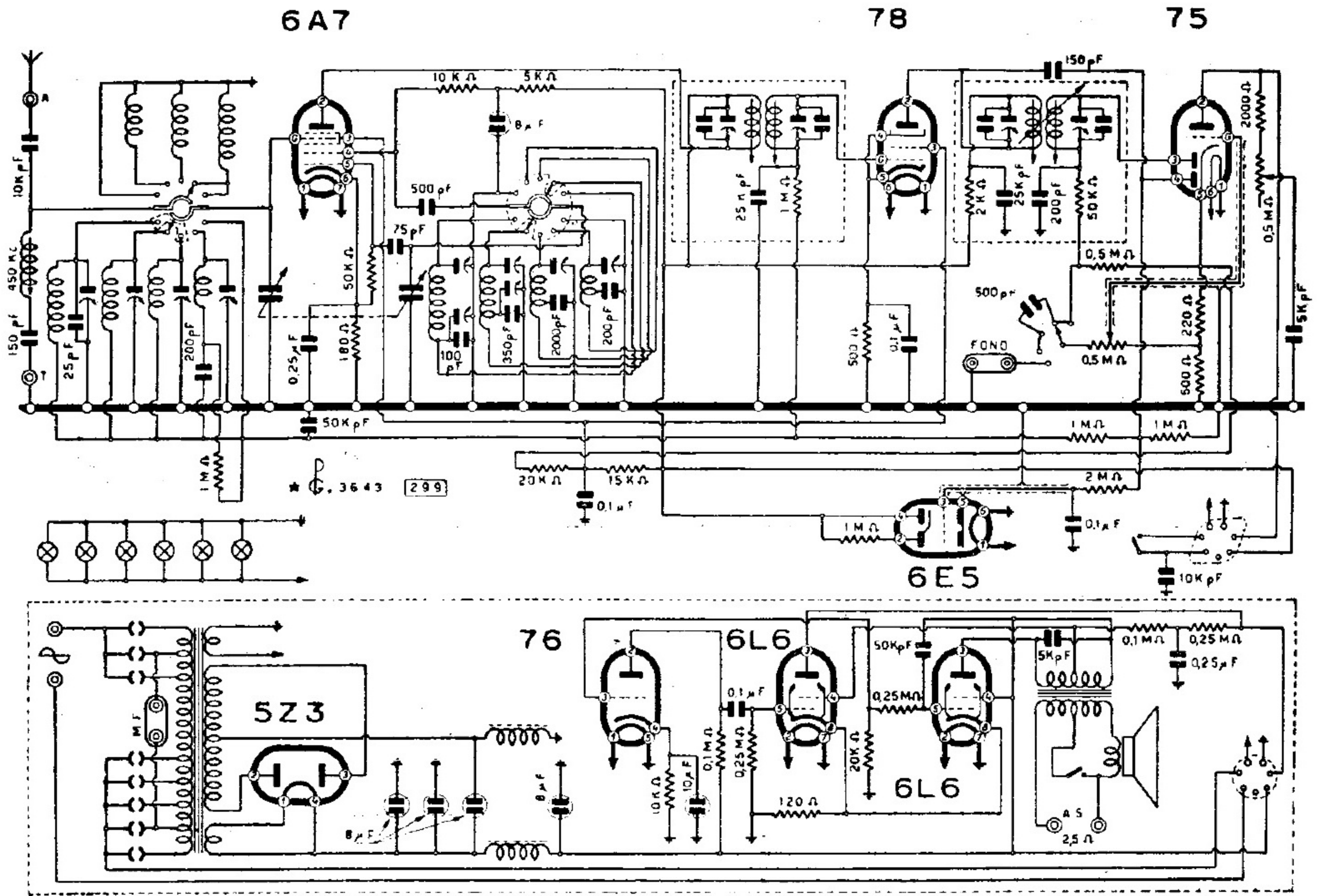
UNDO RADIO - MOD. « SUPER QUADRI UNDA 838 »
