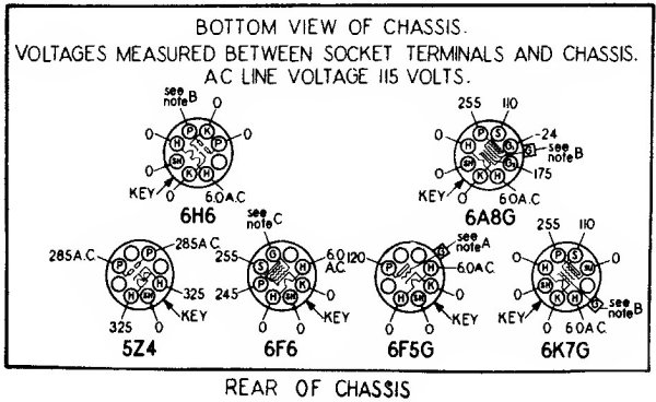
DELCO MODEL R-1117 CIRCUIT DIAGRAM
