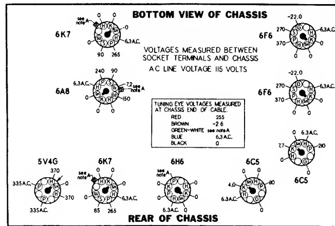
DELCO MODEL R-1118 CIRCUIT DIAGRAM
