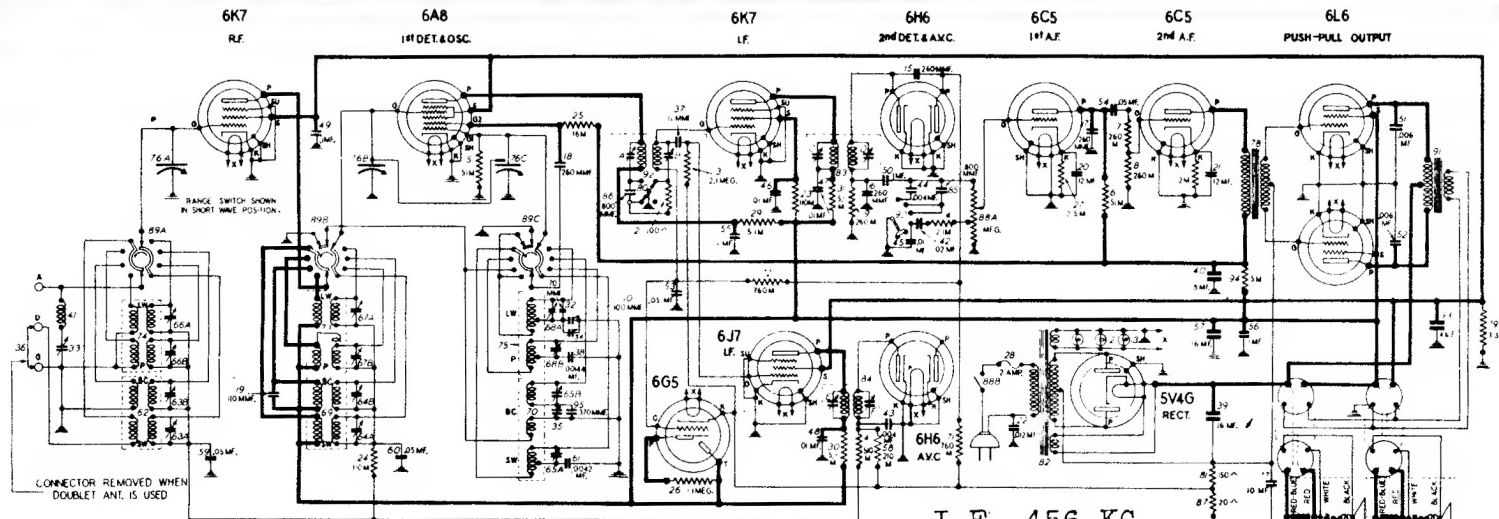
DELCO MODEL R-1119 CIRCUIT DIAGRAM
