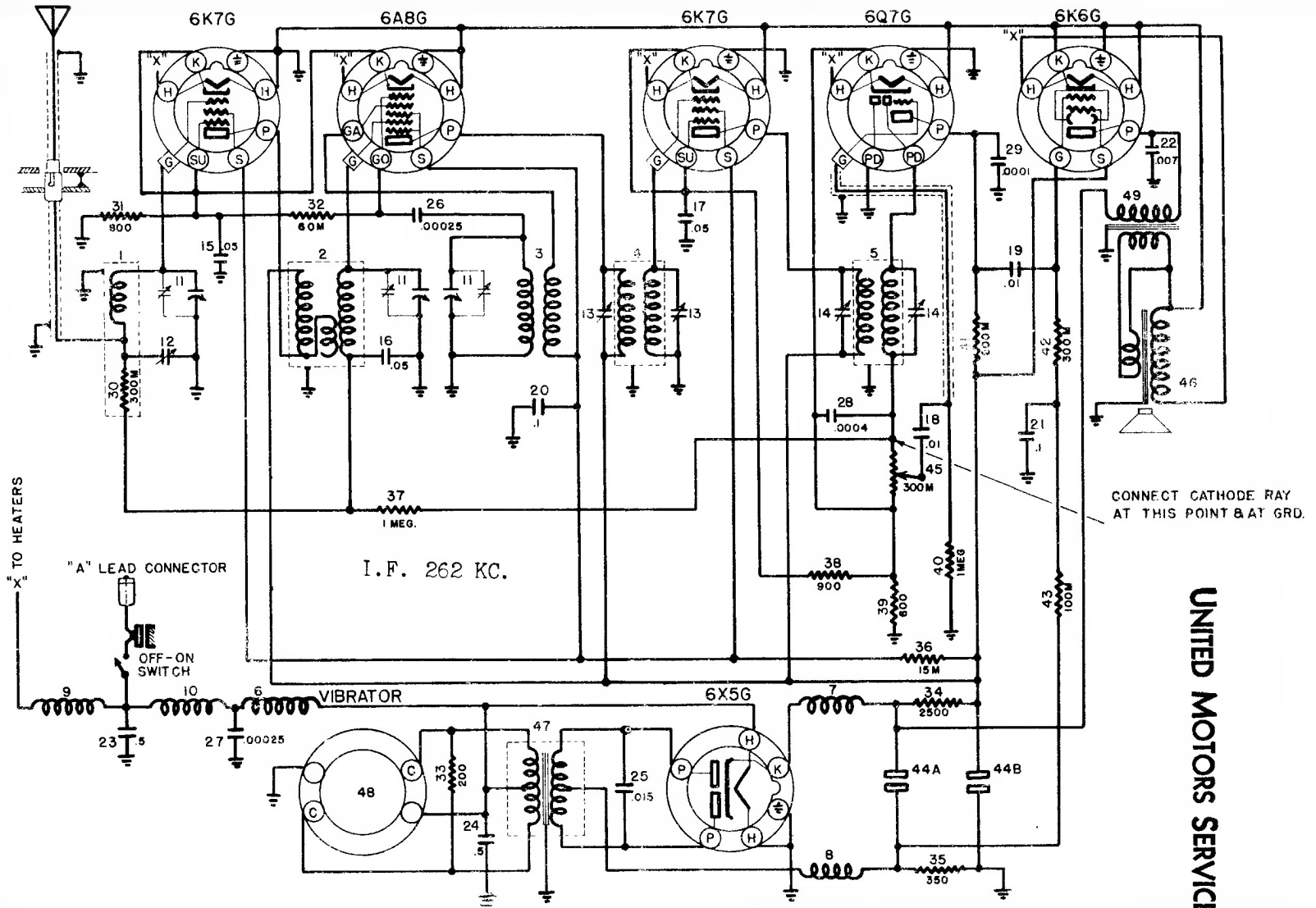
DELCO MODEL R-663 CIRCUIT DIAGRAM
