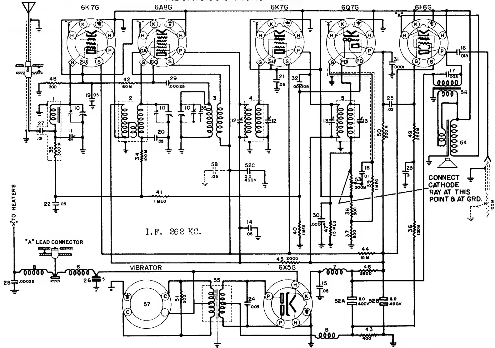
DELCO MODEL R-664 CIRCUIT DIAGRAM
