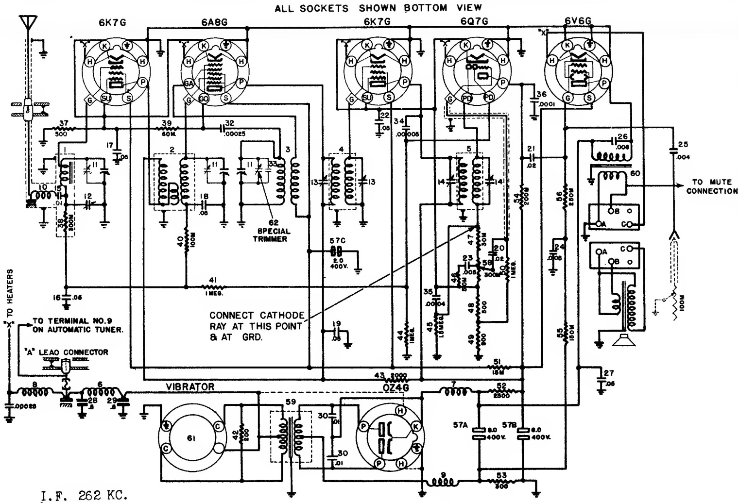
DELCO MODEL R-666-7 CIRCUIT DIAGRAM
