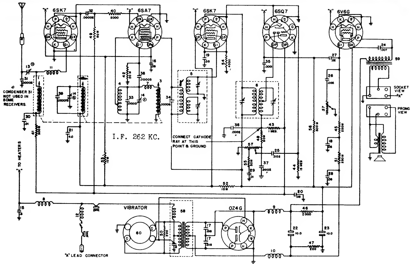
DELCO MODEL R-677 CIRCUIT DIAGRAM
