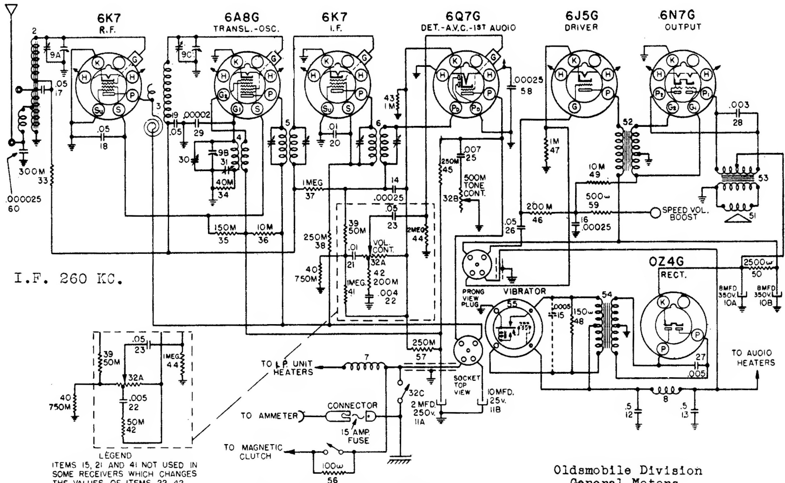
CIRCUIT DIAGRAM OLDS MODEL 982126 4 PRONG CABLE SPEAKER
