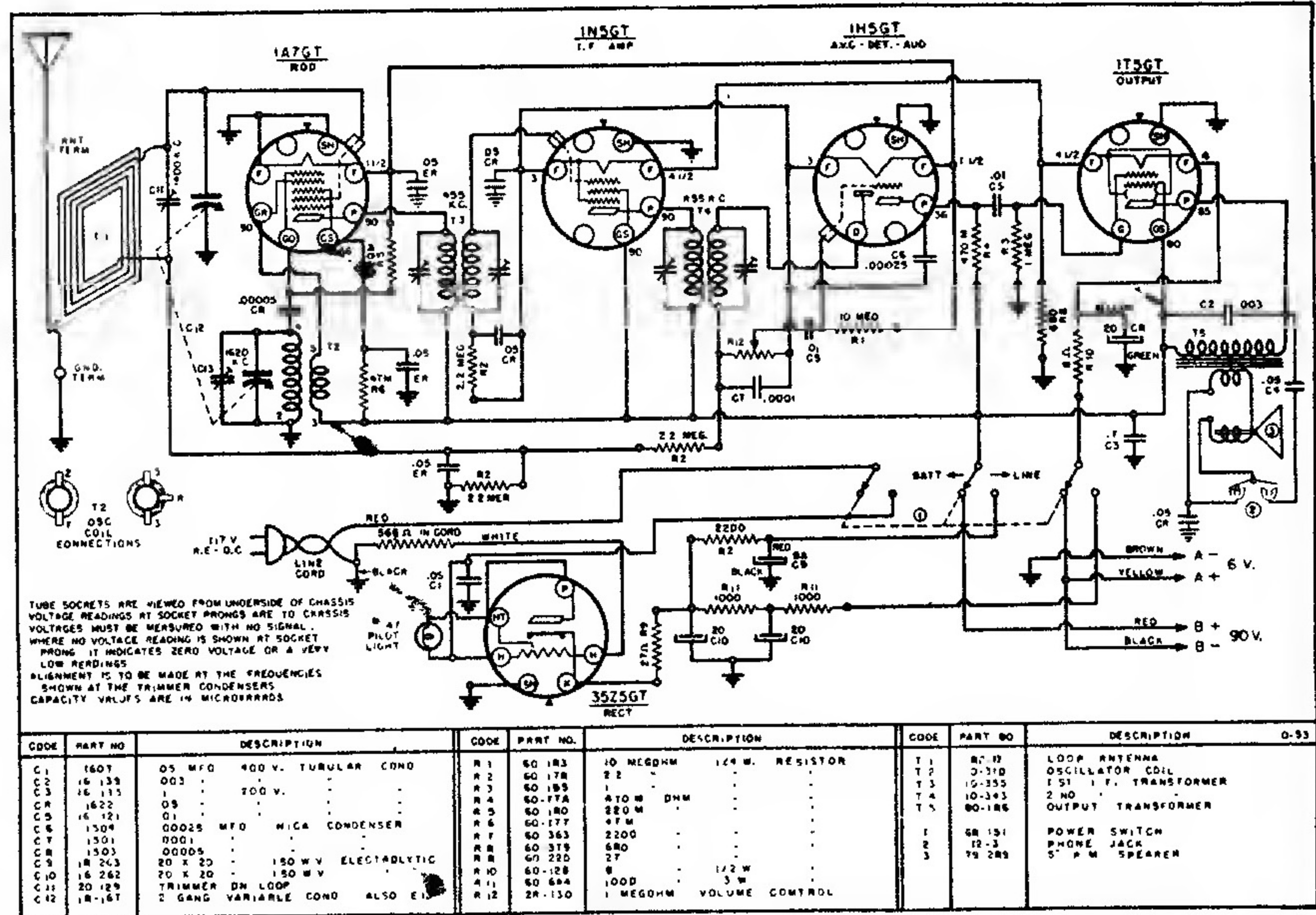
Model No. 0-53 radio receiver
