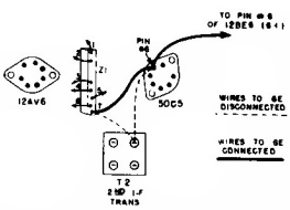
BOTTOM VIEW OF V-2157-4 CHASSIS SHOWING CHANGE TO ELIMINATE "MOTORBOATING"
