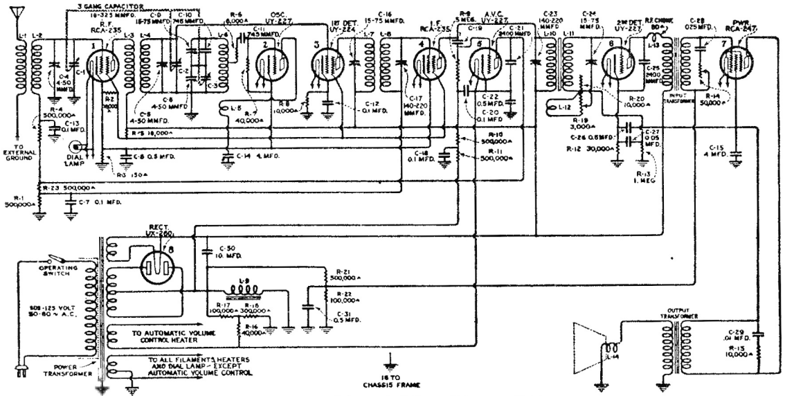
Schematic Wiring Diagram R-10
